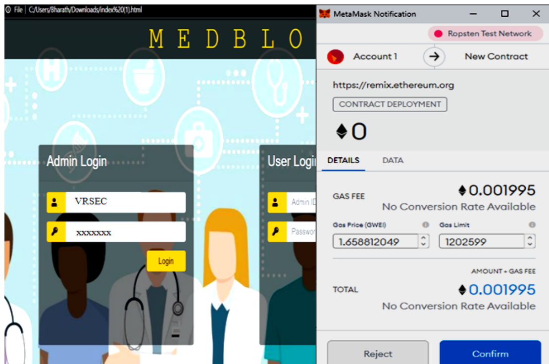
Figure 4. Metamask connection confirmation to process the smart contract over the DApp platform.
