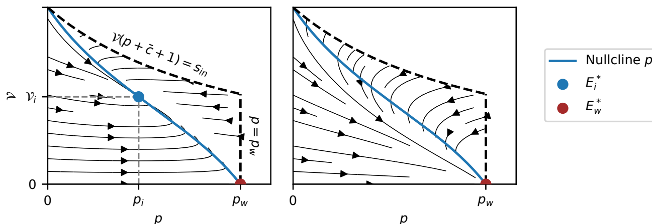
Figure 2. Phase plane of the limiting system S''_1 showing: The case where \bar{\mu}(p_w) \geq D (left), so that the equilibrium E_i^* exists and attracts all solutions; and the case where \bar{\mu}(p_w) < D (right) and E_w^* attracts all solutions.
