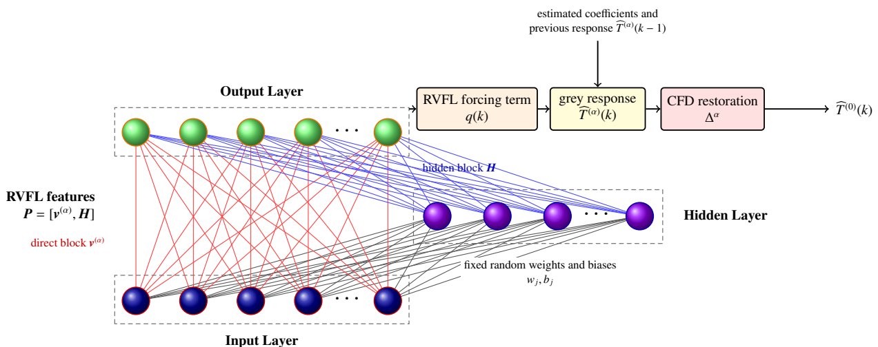
Figure 2. Architecture of CFSRGRVFL. The RVFL component concatenates the direct input block \mathbf{v}^{(\alpha)} and the randomized hidden-feature block \mathbf{H} as \mathbf{P} = [\mathbf{v}^{(\alpha)}, \mathbf{H}] . The resulting forcing term drives the grey response, followed by CFD restoration. The red connections represent the direct input–output link, the blue connections represent the hidden-to-output connections whose coefficients form \beta , and the black connections represent the fixed random input-to-hidden weights and biases w_j and b_j .
