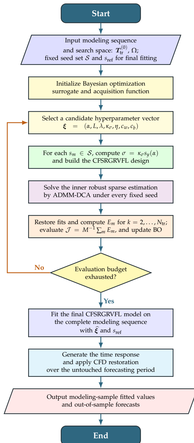
Figure 3. CFSRGRVFL workflow for Bayesian hyperparameter optimization and final model fitting.
