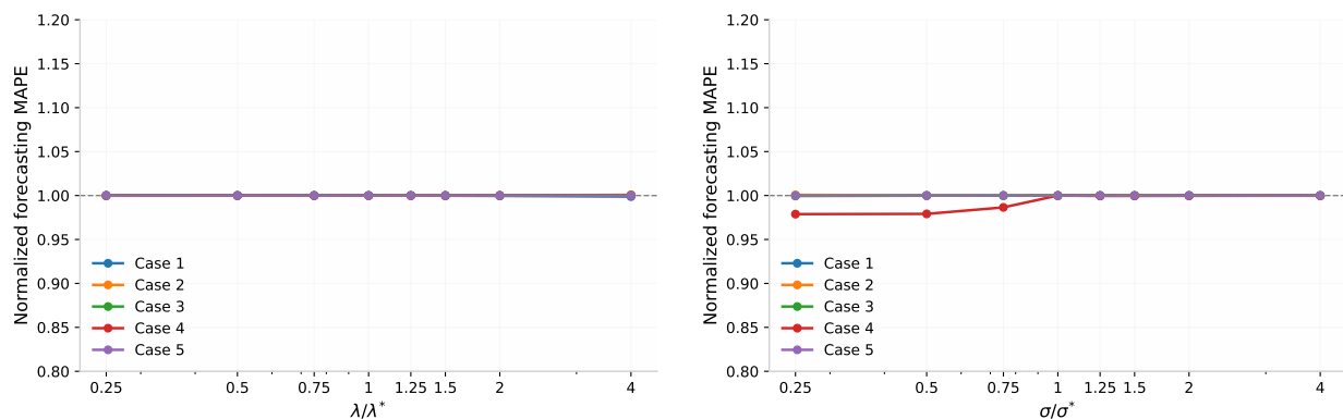
Figure 9. Sensitivity of the forecasting MAPE to (a) \lambda and (b) \kappa_\sigma . The horizontal axis gives the parameter ratio relative to the BO-selected value (log scale); the vertical axis gives the MAPE normalized by its value at ratio 1 (dashed line) and is drawn on a wide scale (0.8–1.2) to show that no hidden fluctuation occurs. The slight dip of Case 4 in panel (b) is associated with its trend reversal, where the loss scale modestly affects the downweighting of large residuals.
