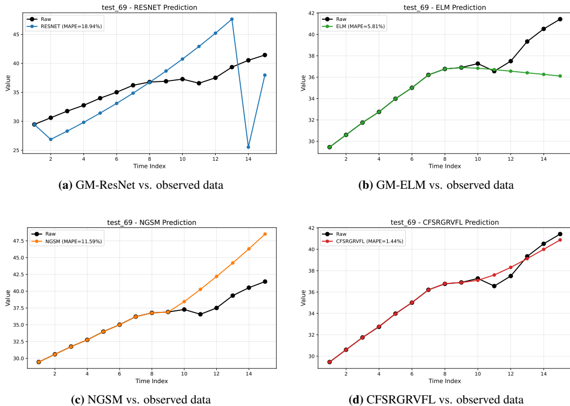
Figure 4. Fitting and forecasting trajectories of the compared neural grey models in Case 1.
