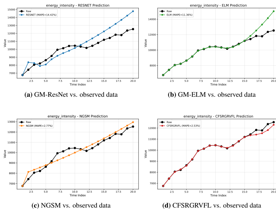
Figure 8. Fitting and forecasting trajectories of the compared neural grey models in Case 5.
