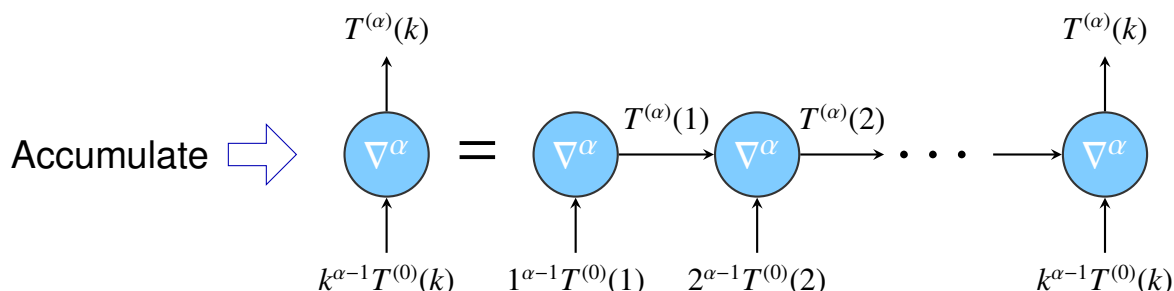
Figure 1. The structure of conformable fractional accumulation.
