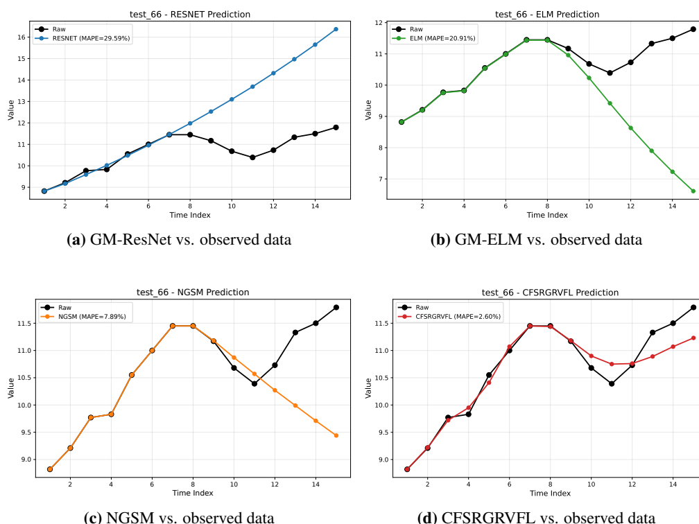
Figure 6. Fitting and forecasting trajectories of the compared neural grey models in Case 3.
