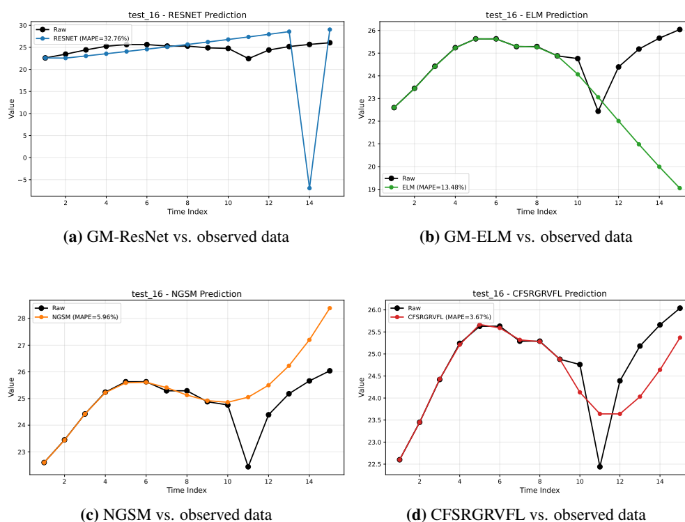
Figure 5. Fitting and forecasting trajectories of the compared neural grey models in Case 2.
