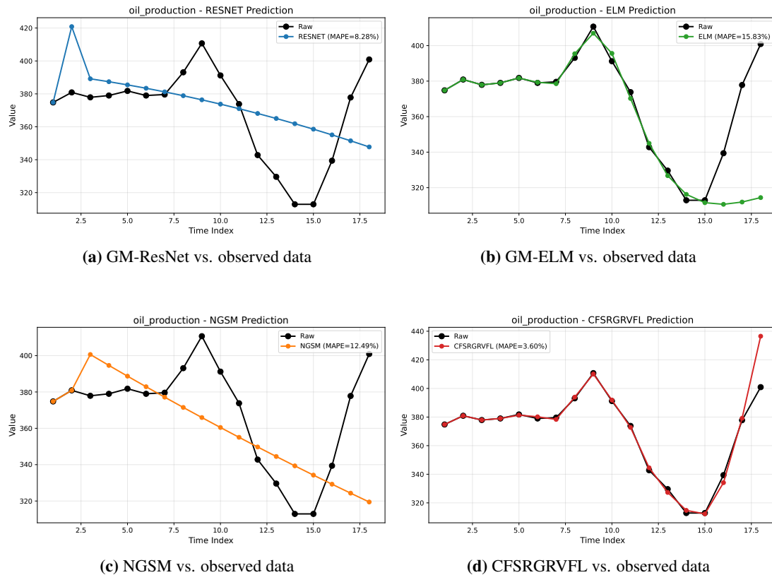
Figure 7. Fitting and forecasting trajectories of the compared neural grey models in Case 4.
