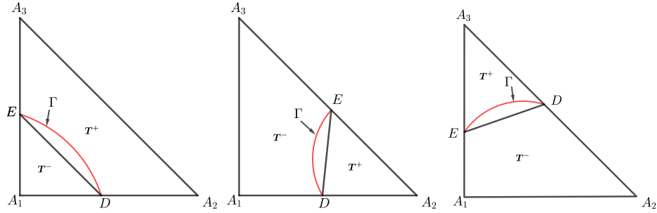
FIGURE 3. Types of interface elements. From left: Type I, Type II, Type III.
