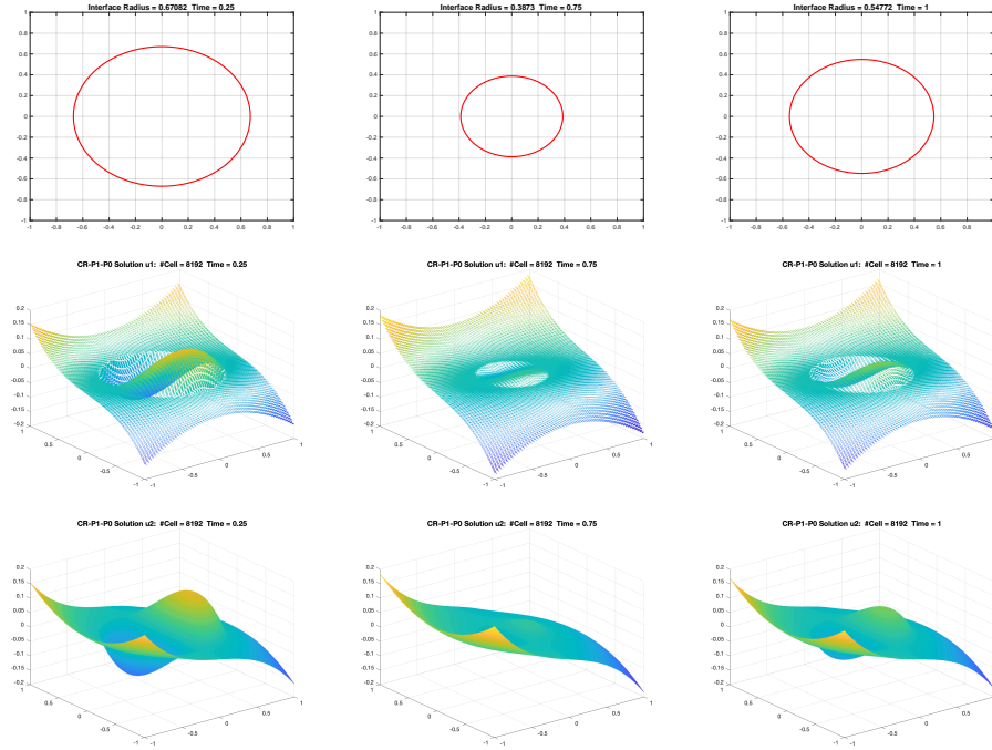
FIGURE 6. CR- P_1 - P_0 IFE Solution of Example 5.3 with \mu^- = 1 and \mu^+ = 10 on the 64 \times 64 mesh at times t = 0.25, 0.75 , and 1 . Top plots: Interfaces, middle: IFE solutions u_{1h} , bottom: IFE solutions u_{2h} .
