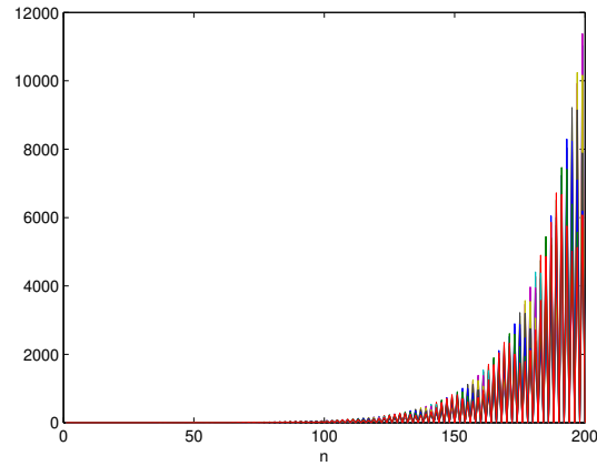
FIGURE 3. The plot of system (23) with A = 0.9 < 1
