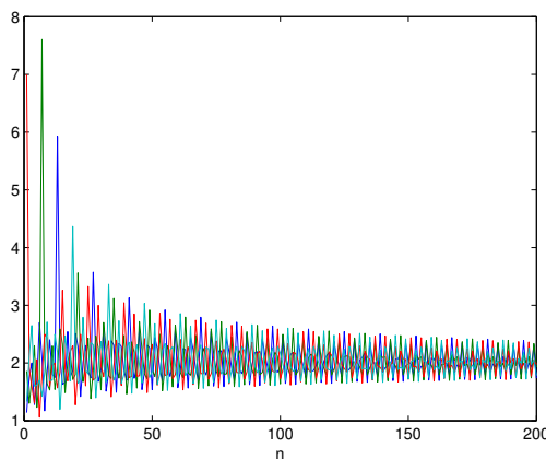
FIGURE 5. The plot of system (24) with A = 1
