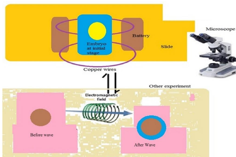
Figure 4. Connecting a battery to a sample of embryonic cells at initial stages ( 100x \times 10x \times 4x = 4000x microscope).
