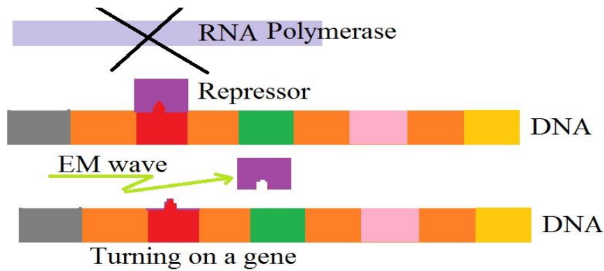
Figure 1. Removing a repressor by a wave.
