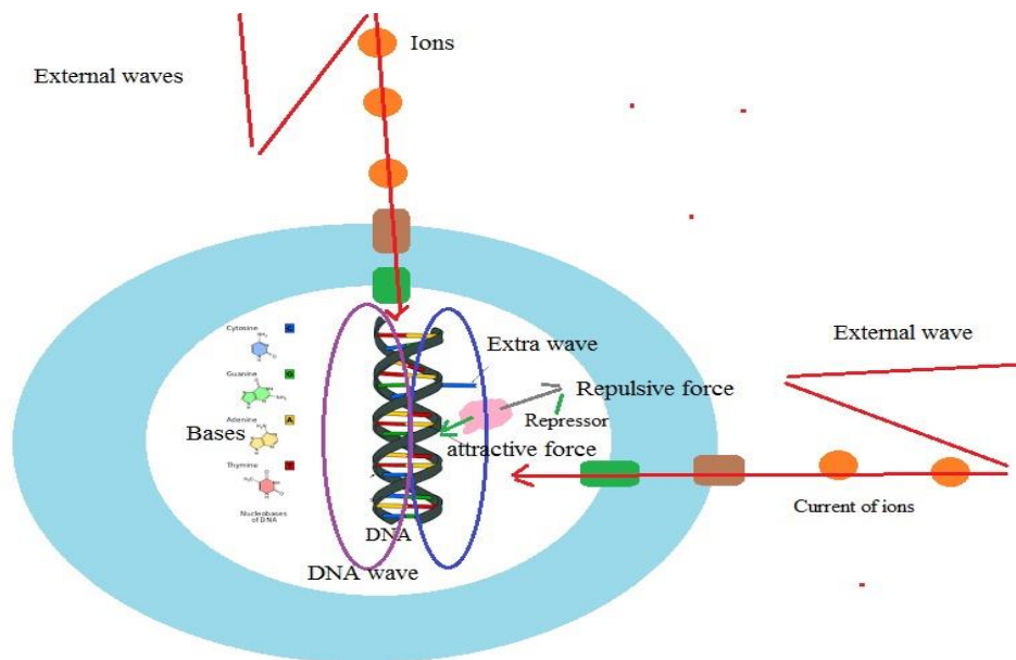
Figure 2. Effect of external waves on exchanged forces and energies between a DNA and a repressor.
