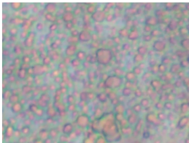
Figure 5. Quail embryonic cells before connecting system to a battery ( 100x \times 10x \times 4x = 4000x microscope).
