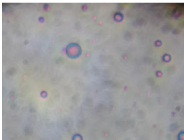
Figure 6. Quail embryonic cells after connecting system to a battery ( 100x \times 10x \times 4x = 4000x microscope).
