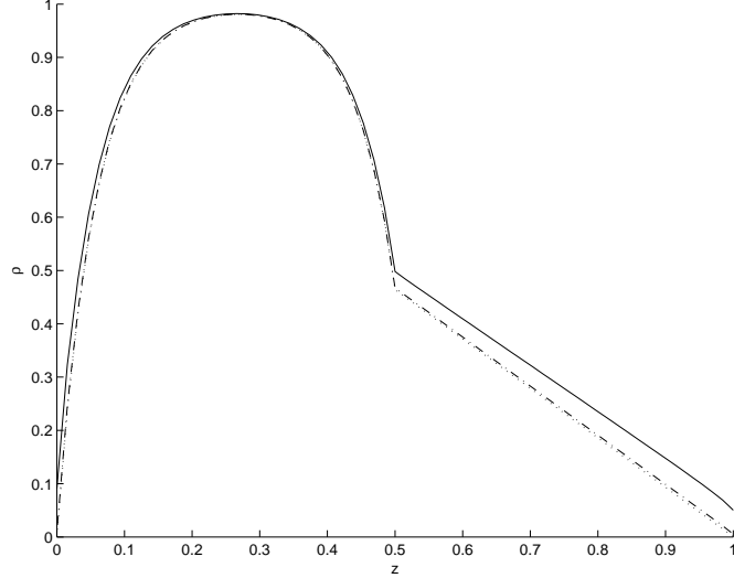
FIGURE 1. Example 1. The numerical solutions of \rho(z) for \epsilon = 0.1, 0.01, 0.001 are plotted by the solid line, dashed line and dotted line respectively.
