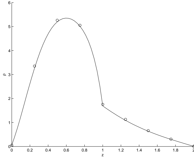
FIGURE 2. Example 2. Numerical solutions of the new method with \Delta z = 1/4 are represented by circles, while the solid line is the 'exact' solution which is calculated by the same numerical method with \Delta z = 1/256
