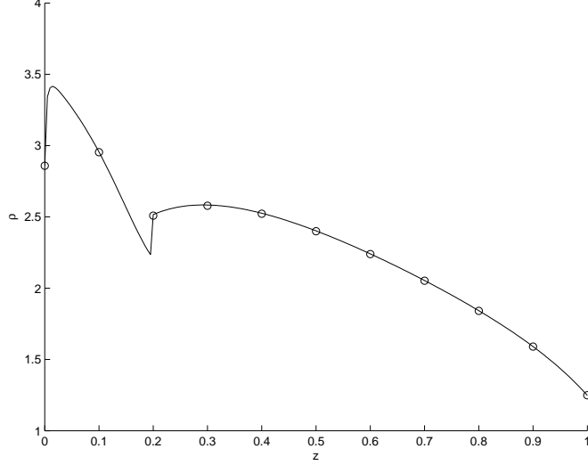
FIGURE 3. Example 3. Numerical solutions of our new method with \Delta z = 1/10 are represented by circles, while the “exact” solution is represented by the solid lines.
