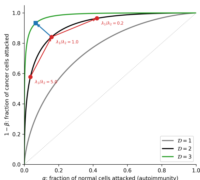
Figure 4. Threshold Shift vs. Discriminability Improvement. ROC curves are plotted for \mathcal{D} = 1, 2, 3 . Increasing \lambda_2 (checkpoint inhibitors) moves the immune system along a fixed ROC curve, increasing cancer cell killing at a cost of increased autoimmunity. Increasing \mathcal{D} (antigen-directed therapies) moves the ROC curve, allowing both type 1 and type 2 errors to decrease.
