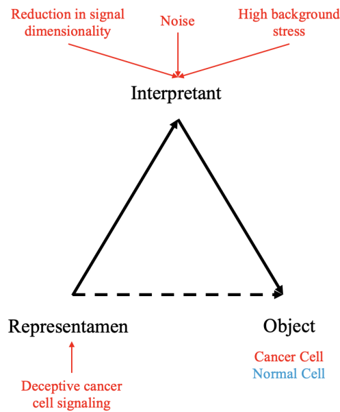
Figure 1. Peirce's triadic model adapted to cancer-autoimmune classification. Reduction in signal dimensionality, noise, and high background stress corrupt the immune interpretant, thus driving a divergence between the dynamical and immediate object. Deceptive cancer cell signaling corrupts the representamen.
