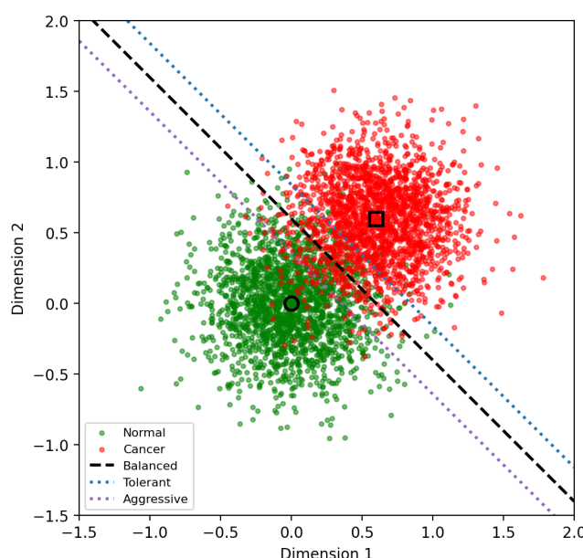
Figure 2. Visualization of overlapping distributions in two-dimensional signal space. 2D signal space showing normal (green) and cancer (red) distributions with three immune classifiers. The dashed line corresponds to the balanced total error minimizer ( \lambda_1/\lambda_2 = 1 ), and the dotted lines correspond to the Bayes-optimal boundaries for aggressive ( \lambda_1/\lambda_2 = 1/5 ) and tolerant classifiers ( \lambda_1/\lambda_2 = 5 ). Overlapping distributions mean that misclassification will occur, regardless of where the classification boundary is set.
