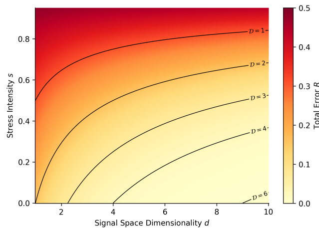
Figure 3. Total error rate and discriminability landscapes. Total error rate increases with stress and decreases with dimensionality. Discriminability decreases with stress and increases with dimensionality.
