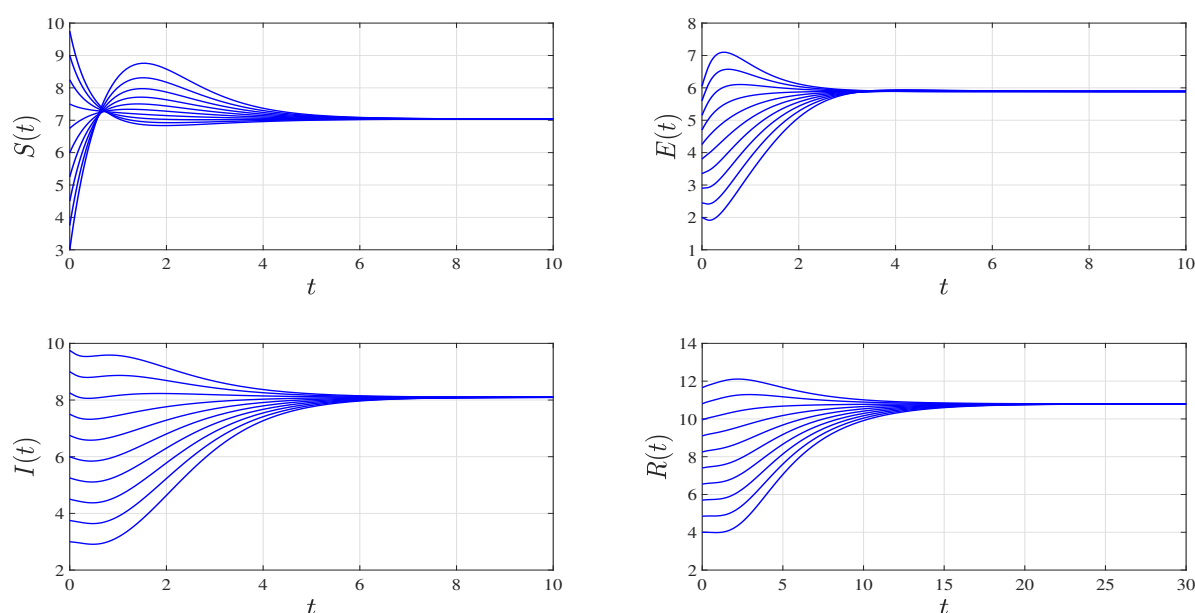
Figure 3. Numerical solutions of the non-delayed avian influenza model (3.1) for different initial bird populations when \mathcal{R}_0 = 11.4583 > 1 .
