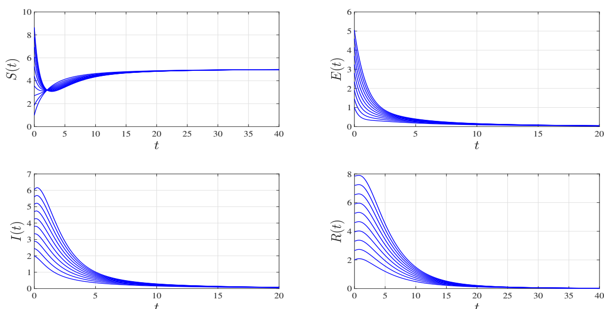
Figure 2. Numerical solutions of the non-delayed avian influenza model (3.1) for different initial bird populations when \mathcal{R}_0 = 0.859 < 1 .
