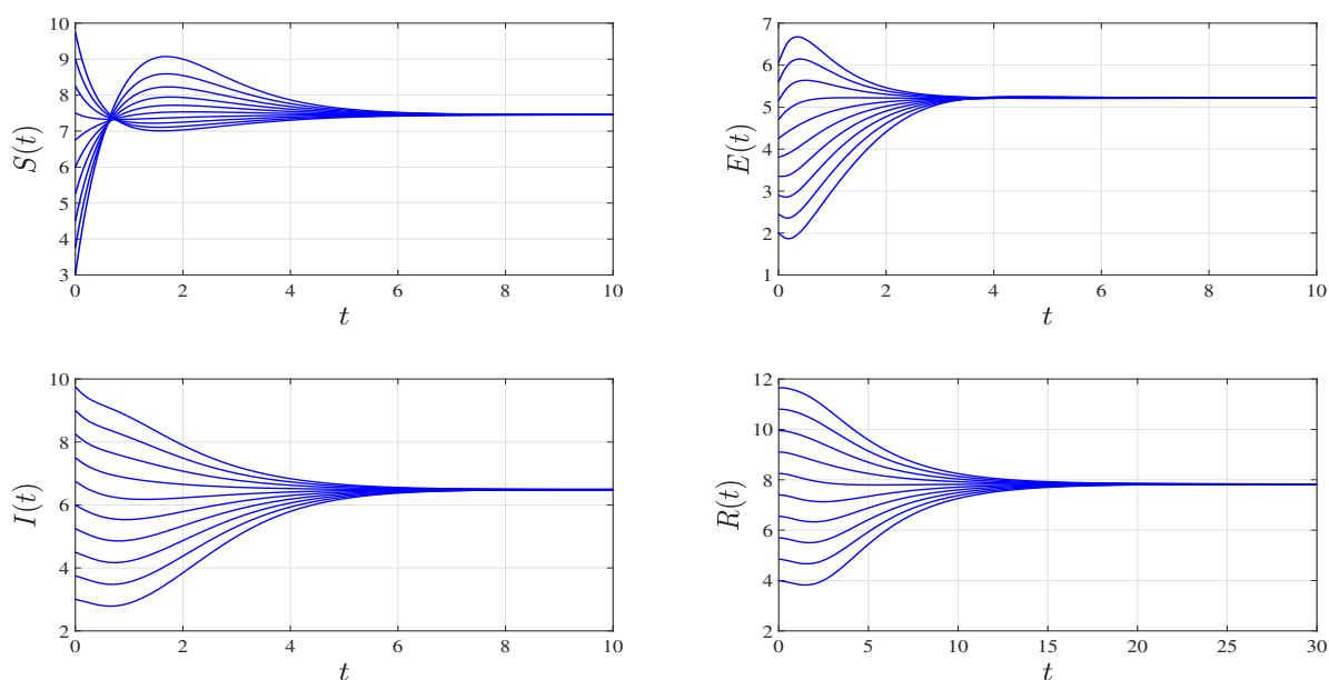
Figure 5. Numerical solutions of the delayed avian influenza model (5.1) for different initial conditions when \mathcal{R}_d = 9.381 > 1 .
