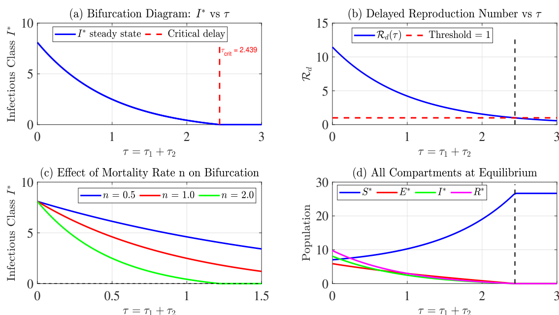
Figure 8. Bifurcation diagram of the infectious class I^* at equilibrium as a function of the total delay \tau = \tau_1 + \tau_2 , with \tau_1 = \tau_2 = \tau/2 .
