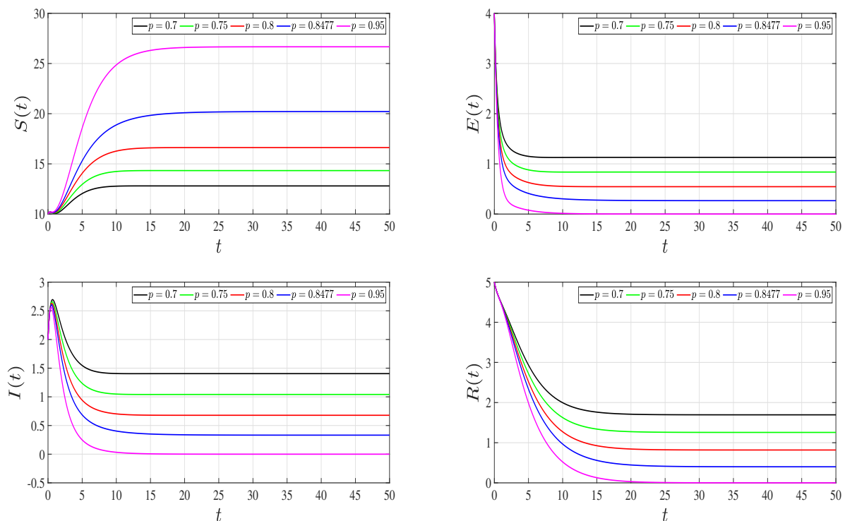
Figure 7. Effect of infection-blocking control efficacy p on the four bird classes in the delayed avian influenza model.
