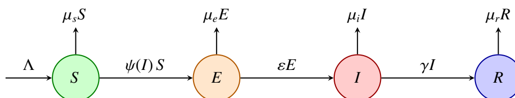
Figure 1. Flow diagram of the avian influenza transmission model in a bird population.
