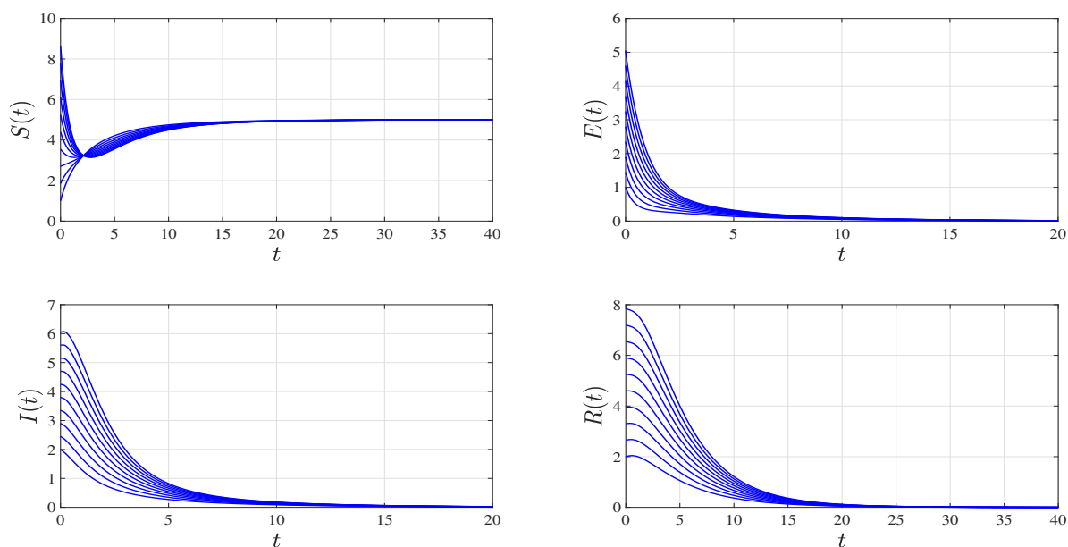
Figure 4. Numerical solutions of the delayed avian influenza model (5.1) for different initial conditions when \mathcal{R}_d = 0.704 < 1 .
