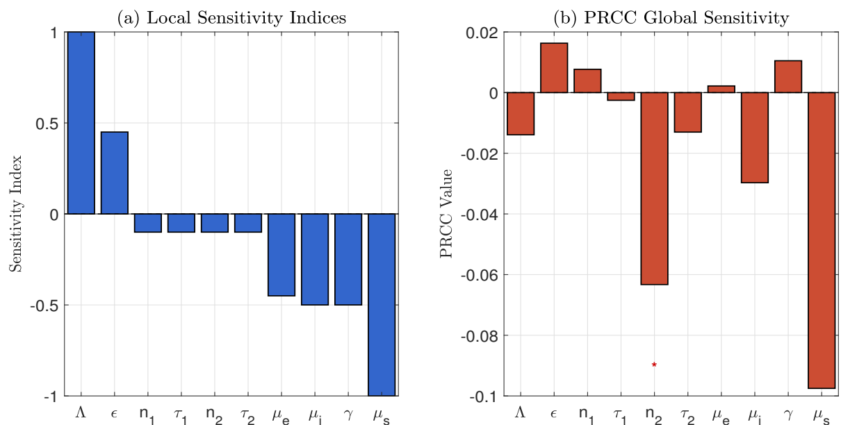
Figure 6. Local sensitivity indices and PRCC values of \mathcal{R}_d with respect to the main parameters of the delayed avian influenza model.
