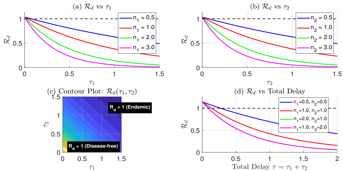
Figure 9. Variation of the delayed basic reproduction number \mathcal{R}_d with respect to time delays. (a) \mathcal{R}_d as a function of \tau_1 for different values of n_1 , with \tau_2 = 0.1 and n_2 = 1 . (b) \mathcal{R}_d as a function of \tau_2 for different values of n_2 , with \tau_1 = 0.1 and n_1 = 1 . (c) Contour plot of \mathcal{R}_d as a function of both \tau_1 and \tau_2 with n_1 = n_2 = 1 .
