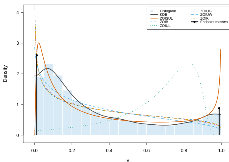
Figure 2. Fitted density curves of six zero–one-inflated unit-interval models for the empirical data.
