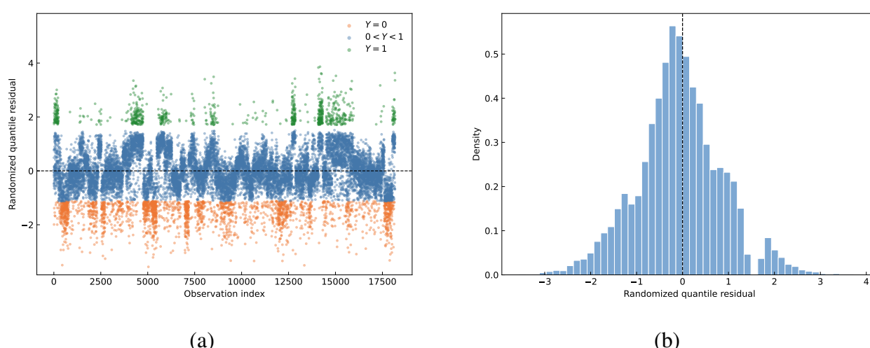
Figure 3. Randomized quantile residual diagnostics for the ZOISUL model fitted to the PROPAT7 data: (a) Residual scatterplot in the original record order; (b) Residual histogram.
