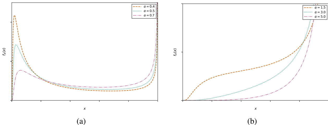
Figure 1. Probability density functions of the \text{SUL}(\alpha) distribution for selected parameter values: (a) 0 < \alpha < \alpha_0 ; (b) \alpha \geq \alpha_0 .
