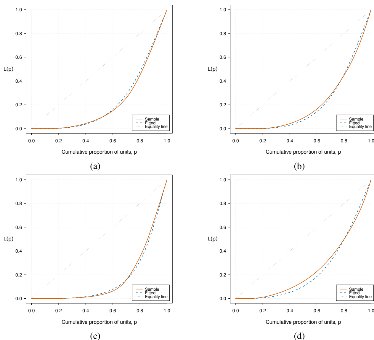
Figure 4. Sample and fitted Lorenz curves for the proportion of teachers with an ISCED Level 7 qualification across different school groups: (a) Public rural schools; (b) Private rural schools; (c) Public urban schools; (d) Private urban schools.
