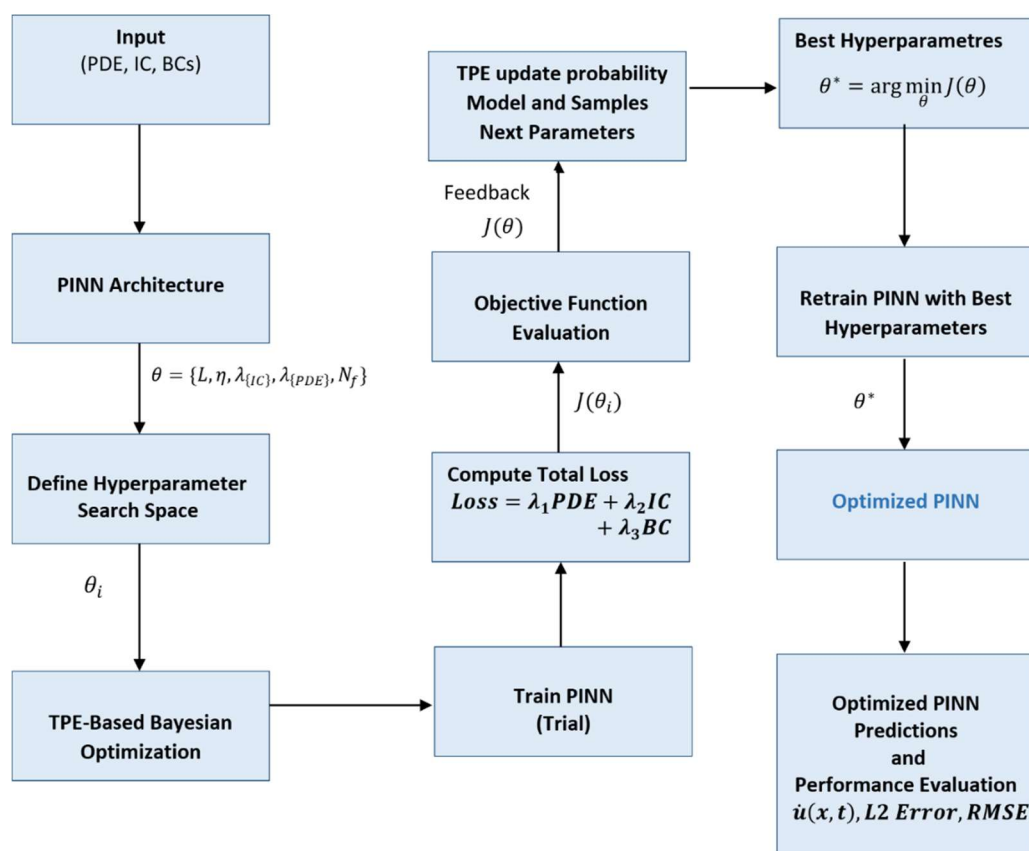
Figure 1. TPE-based Bayesian optimization architecture.
