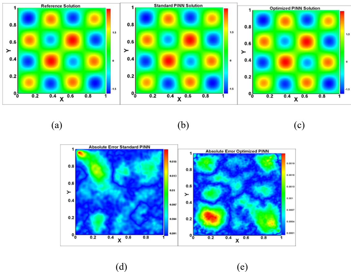
Figure 10. Nonlinear elliptic two-dimensional equation: (a) Reference solution, (b) Standard PINN solution, (c) Optimized PINN solution, (d) Absolute error standard PINN, (e) Absolute error optimized PINN.
