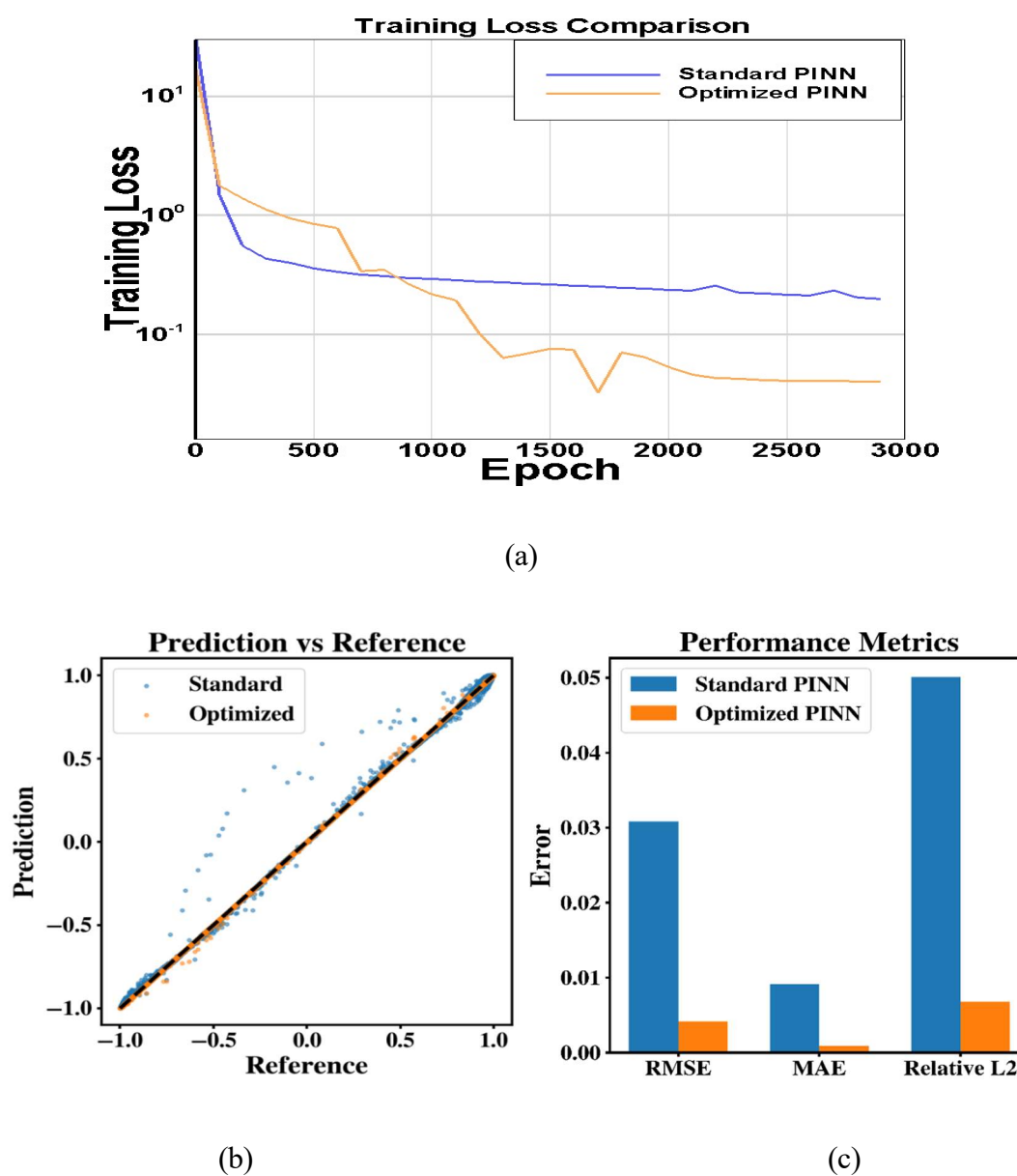
Figure 4. (a) Training loss curves of standard and optimized PINN. (b) Prediction vs reference solution. (c) Performance metrics.
