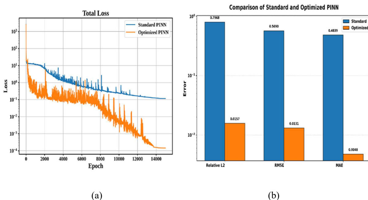
Figure 8. (a) Training loss curves of standard and optimized PINN. (b) Performance metrics.
