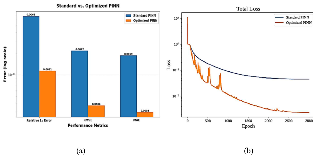
Figure 11. (a) Performance metrics of standard and optimized PINN (b) Training loss curves of standard and optimized PINN.
