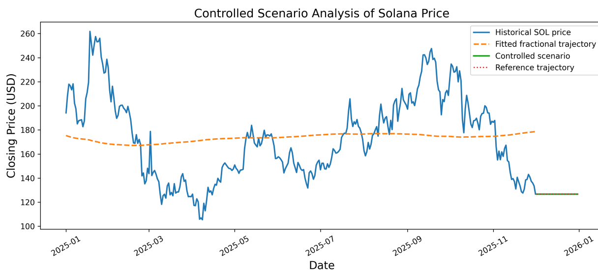
Figure 7. Controlled scenario analysis of the Solana price using the fractional impulsive VFIDE framework. The controlled trajectory is compared with the historical and fitted trajectories and a prescribed reference trajectory.
