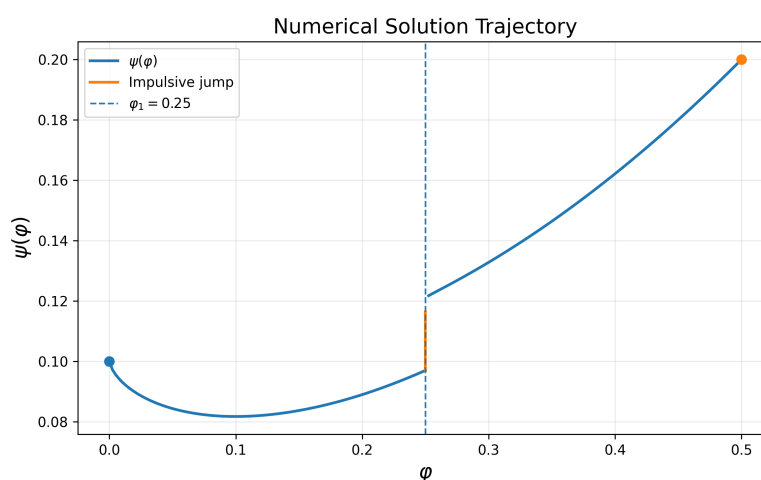
Figure 1. Numerical solution trajectory \psi(\varphi) with the impulsive jump at \varphi_1 = 0.25 .
