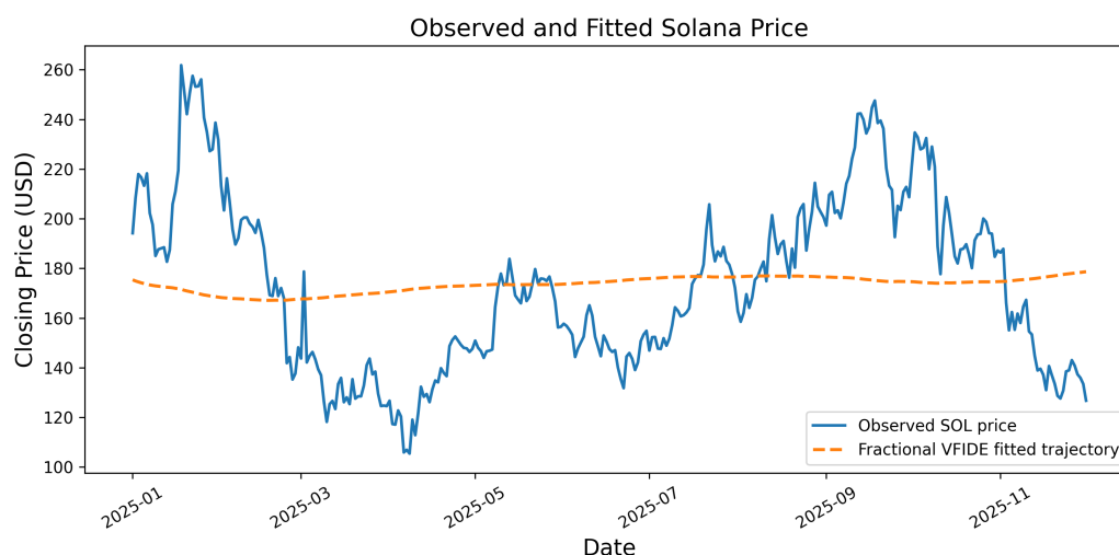
Figure 6. Comparison between the observed Solana closing price and the trajectory fitted using the proposed fractional impulsive VFIDE model.
