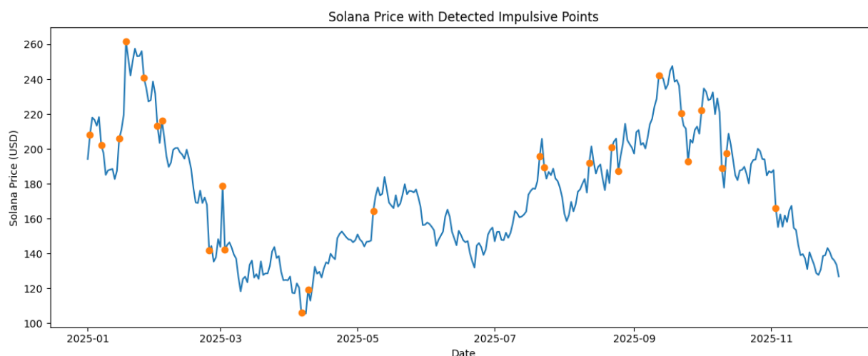
Figure 5. Solana closing-price trajectory with the detected impulsive points marked in red according to the prescribed price-change threshold.
