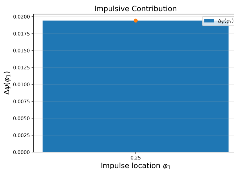
Figure 2. Computed impulsive contribution \Delta\psi(\varphi_1) at the impulse point \varphi_1 = 0.25 .
