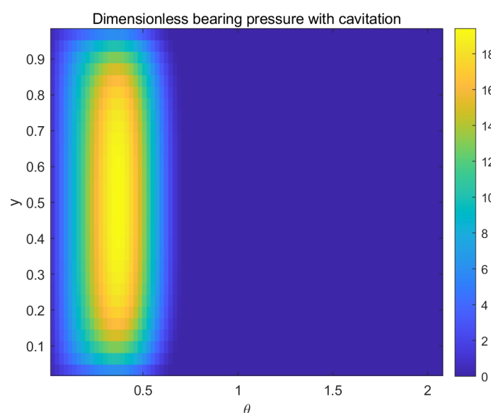
Figure 5. Dimensionless Reynolds pressure at \varepsilon = 0.9 on the 90 \times 30 grid. Color represents the pressure p .
