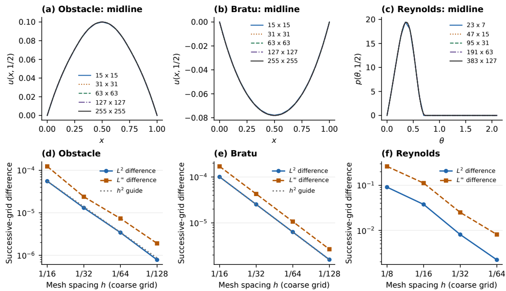
Figure 7. Field-level mesh-convergence checks. Top row: Displacement or pressure along the physical midline y = 1/2 , with zero boundary values included; legend entries are interior grid dimensions. Bottom row: Discrete L^2 and infinity-norm differences between adjacent residual-checked grids, evaluated at coincident nodes. The bottom-row horizontal axes run toward finer meshes. The guides in (d) and (e) indicate an h^2 slope only. No exact continuum field is assumed.
