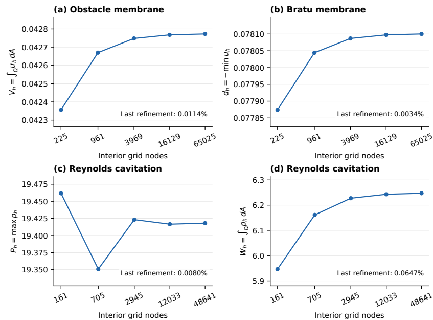
Figure 6. Physical-output grid-convergence study with five meshes per model. The abscissa is the number of interior nodes on a logarithmic scale. Panels show (a) the obstacle displacement integral, (b) the Bratu maximum downward deflection, (c) the Reynolds peak pressure, and (d) the sector pressure integral. Annotations give the last relative refinement change. Lines connect computed values only. The post-solve accuracy check and the original Bratu stopping-test exception are described in the text.
