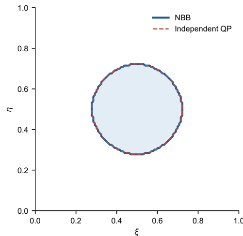
Figure 8. Auxiliary cross-solver check: Active-contact contours obtained with NBB and an independently solved quadratic program at N = 127 , in physical coordinates. The two node classifications agree at the 10^{-7} gap threshold. These are discrete numerical boundaries, not the analytical-solution comparison, which is provided separately in Section 5.3.5.
