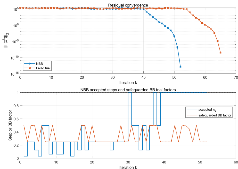
Figure 1. Convergence profile for the illustrative nonconvex WCP instance. The upper panel compares residual decay for NBB and the fixed-trial variant. The lower panel shows the accepted step length and safeguarded BB trial factor used by NBB.
