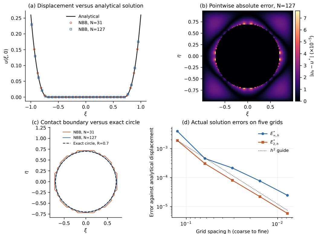
Figure 9. Comparison with the analytical obstacle solution of Harasim and Valdman [39]. (a) Analytical midline displacement and computed nodal values; markers on the N = 127 grid are subsampled for visibility. (b) Actual absolute nodal error at N = 127 . (c) Numerical contact contours and the exact circle r = 0.7 , using physical domain coordinates. (d) Displacement errors relative to the analytical field on five grids. The h^2 line is a slope guide anchored at the coarsest E_{2,h}^* , not a fitted bound or a claim of uniform second-order behavior. All quantities are nondimensional.
