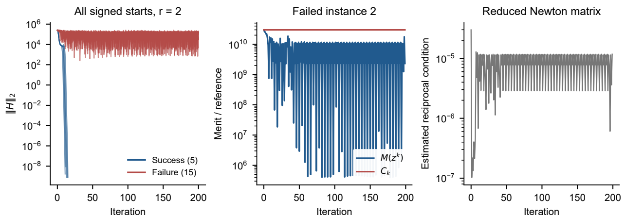
Figure 4. Signed-start Bratu diagnostics at r = 2 . Left: All 20 residual trajectories, including the five successes and 15 failures. Middle: The merit and reference values for failed instance 2. Right: The reciprocal-condition estimate for that instance. Diagnostics stop at the original 200-iteration budget; extended-budget outcomes are reported in the text.
