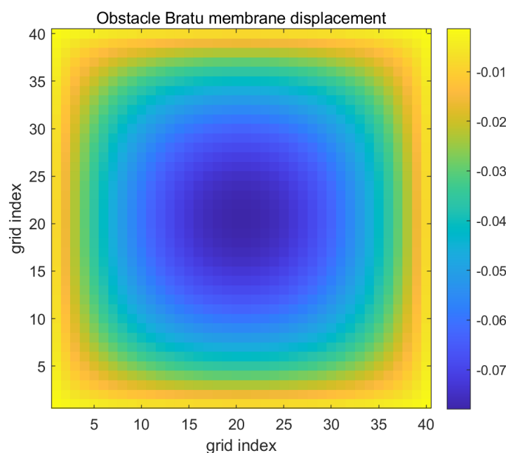
Figure 3. Computed displacement field for the obstacle Bratu membrane on the 40 \times 40 interior grid. The color scale represents the membrane displacement u ; the most negative displacement occurs near the center.
