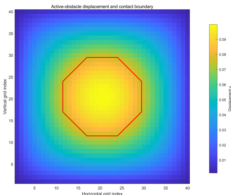
Figure 2. Computed displacement field for the active obstacle problem on the 40 \times 40 interior grid. Color represents the displacement u , and the red contour marks the boundary of the active contact region.
