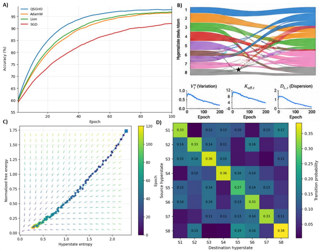
Figure 2. Comprehensive visualization of the optimization dynamics of the proposed study. (A) Convergence comparison of QISGHO with conventional optimization. (B) Evolution of hyperstate probability flow and variation, effective curvature, and dispersion during optimization. (C) Entropy-free energy phase-space trajectory. (D) Hyperstate transition probability matrix representing probabilistic.
