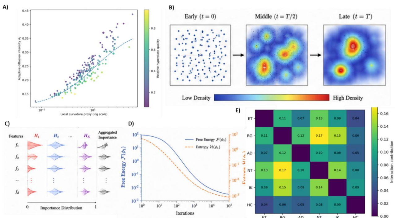
Figure 3. Qualitative visualization of the proposed framework's core optimization mechanisms. (A) Relationship between estimated local curvature and adaptive diffusion intensity. (B) Evolution of the hyperstate probability density. (C) Hyperstate-aware probabilistic feature importance distributions. (D) Joint evolution of the variational free-energy functional and entropy during optimization. (E) Synergistic interaction matrix.
