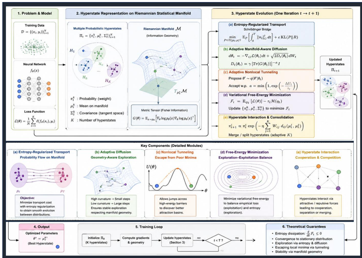
Figure 1. Model architecture of the proposed study.
