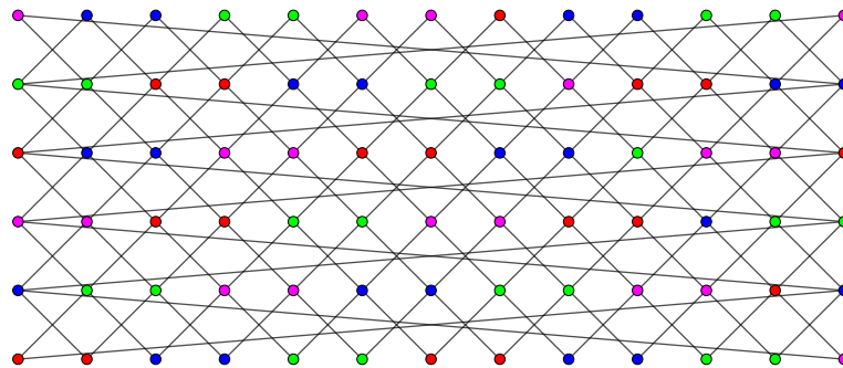
Figure 9. 3-dynamic proper 4-coloring of the direct product P_6 \times C_{13} .
