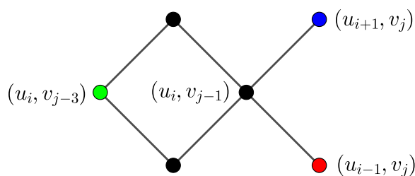
Figure 5. Illustration of Lemma 11.
