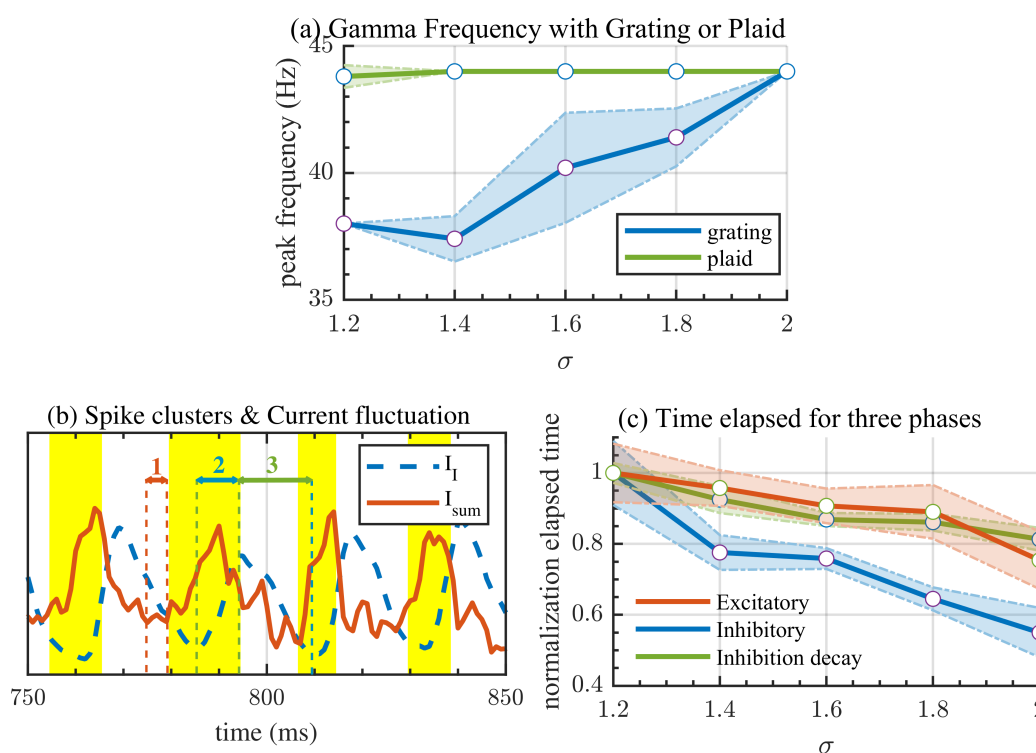
Figure 5. Modulation effect of push-pull strength on peak frequency of gamma oscillation. (a) The trend of peak frequency changes when 50% vertical grating (blue) and 50% vertical + 50% horizontal grating superimposed on plaid (green) are the stimuli. (b) Relationship between firing cluster events (yellow bars) and fluctuations in normalized input currents (blue: inhibitory current; red: total current) of E neurons. The three phases are identified by arrows and numbers in the corresponding colors. (c) Change in elapsed time (normalized) for the excitation phase (red), the inhibition phase (blue), and the inhibition decay phase (green) of the network when 50% vertical grating is used as the visual stimulus. The solid line in (a) and (c) stands for the average of five independent experiments, while the light-colored area surrounded by the dotted line shows the standard deviation.
