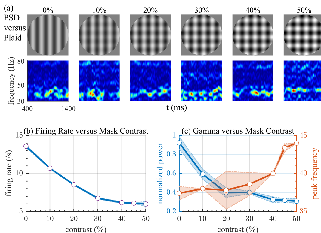
Figure 2. Firing activity with grating and plaids as visual stimuli. (a) Oscillatory PSD analysis of vertical preference populations at different contrasts of horizontal mask gratings. (b) Cross-inhibition during contrast enhancement of horizontal mask gratings. (c) Band power (blue line on the left axis) and peak frequency (red line on the right axis) of gamma oscillation modulated by horizontal grating contrast. The solid line stands for the average of five independent experiments, while the light-colored area surrounded by the dotted line shows the standard deviation.
