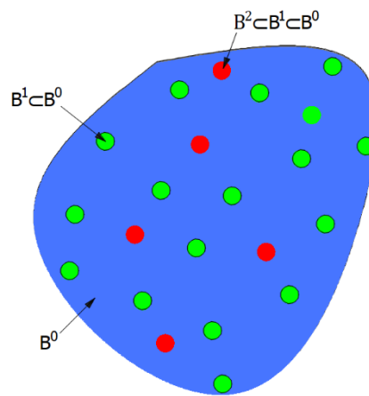
Figure 2. A Peridynamic body showing model levels 0, 1 and 2.
