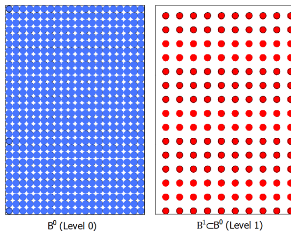
Figure 14. Discretisation and coarsening of the two-dimensional homogeneous plate.
