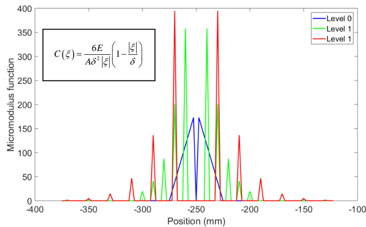
Figure 5. Micromodulus function associated with a bond constant function having triangular profile.
