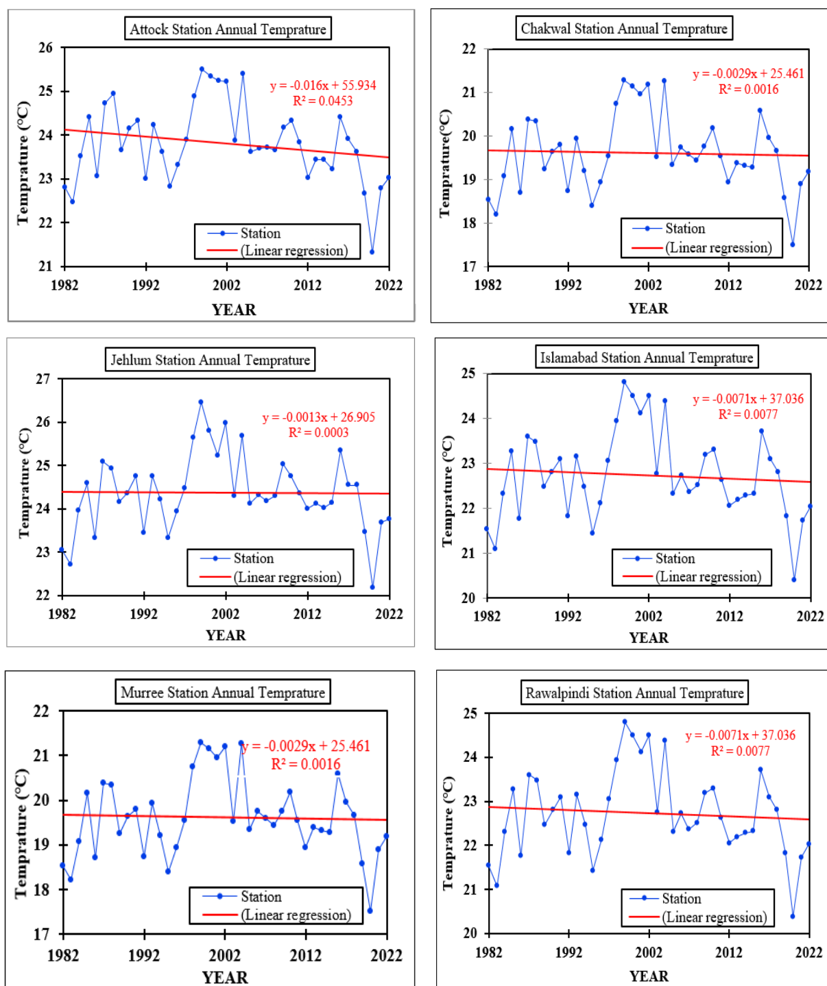
Figure 3. Annual mean temperature variations for six meteorological stations (Attock, Chakwal, Jhelum, Islamabad, Murree, and Rawalpindi) in the Potwar Plateau region from 1982 to 2022. Linear regression lines show slight declining trends at all stations with very low R^2 values, indicating weak relationships. Overall, the figure reflects notable interannual variability and no statistically significant long-term temperature trends across the study area.
