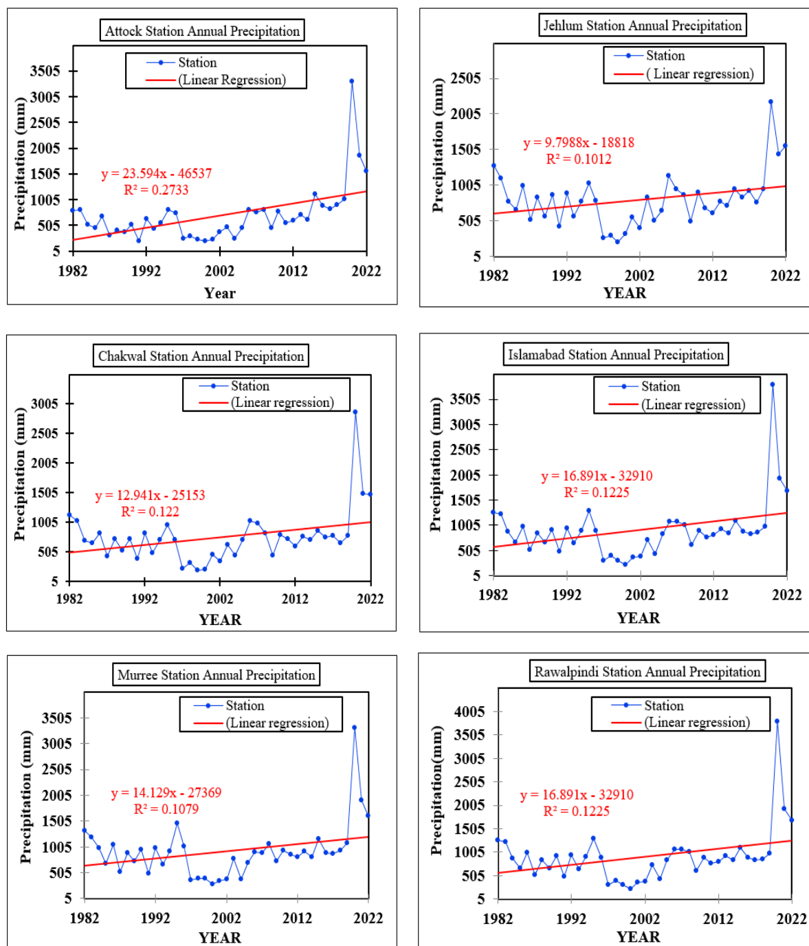
Figure 6. Linear regression of annual precipitation at six meteorological stations (Attock, Chakwal, Jhelum, Islamabad, Murree, and Rawalpindi) from 1982 to 2022. The results show high interannual variability with generally weak trends, as indicated by low R^2 values. A noticeable increase in precipitation is observed after 2015, with a regional peak in 2021 across all stations.
