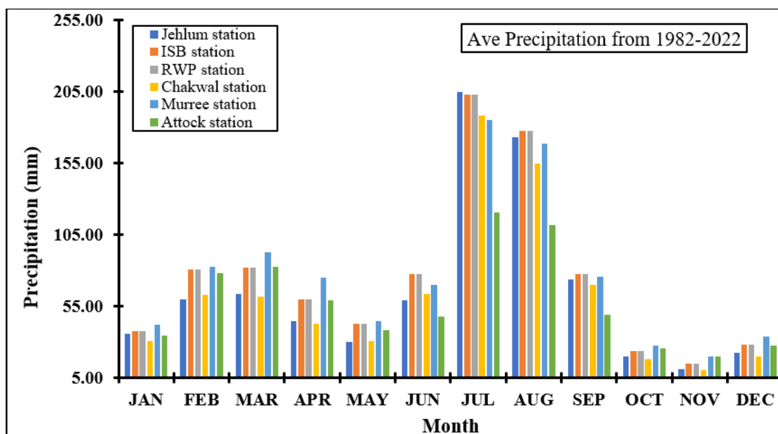
Figure 5. Average monthly precipitation at six meteorological stations (Jhelum, Islamabad, Rawalpindi, Chakwal, Murree, and Attock) in the Potwar Plateau region. Precipitation exhibits strong seasonal variability, with peaks during the monsoon months and lower values in winter. Murree generally records higher precipitation due to elevation, while other stations show relatively similar patterns.
