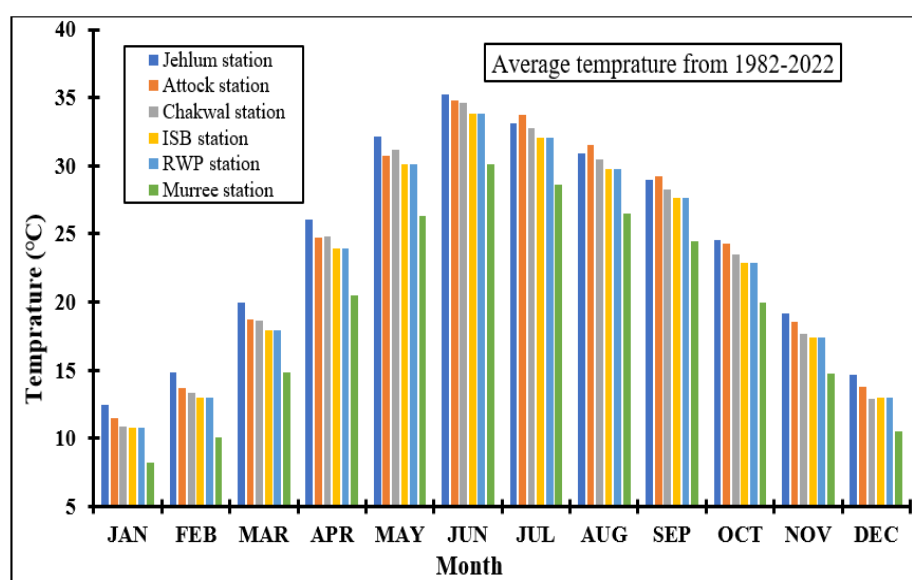
Figure 2. Monthly average temperatures for six stations in the Potwar Plateau (1982–2022). Temperatures rise from winter to a peak in June–July and decline toward December. Murree remains cooler due to its higher elevation, while other stations show similar seasonal patterns.
